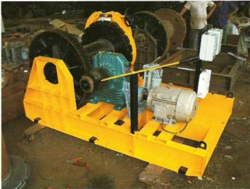
Double Drum Power Winch Capacity : 3 MT, 5 MT, 7.5 MT
