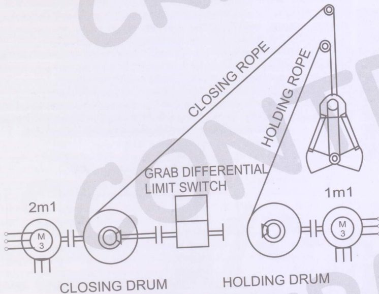
FIG.2 PRINCIPLE OF A CLUTCHLESS TWO DRUM
