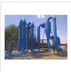
Biomass Briquetting Dryer
