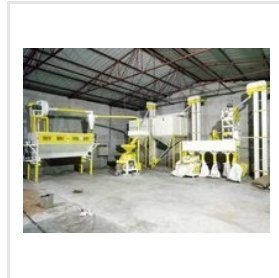
FLOUR MILL PLANT 1TON /HR
