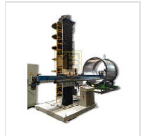
Tank Polishing Machine
