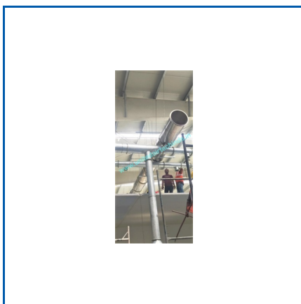
INDUSTRIAL DUCTING SPLIT PIECE SS DUCTING WITH AIR VENTILATION GRILLS PAINT BOOTH EXHAUST SYSTEM
