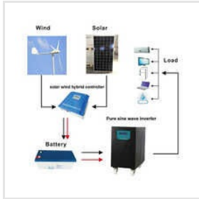
Industrial Solar Hybrid System
