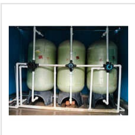
Fluoride Removal Plant
