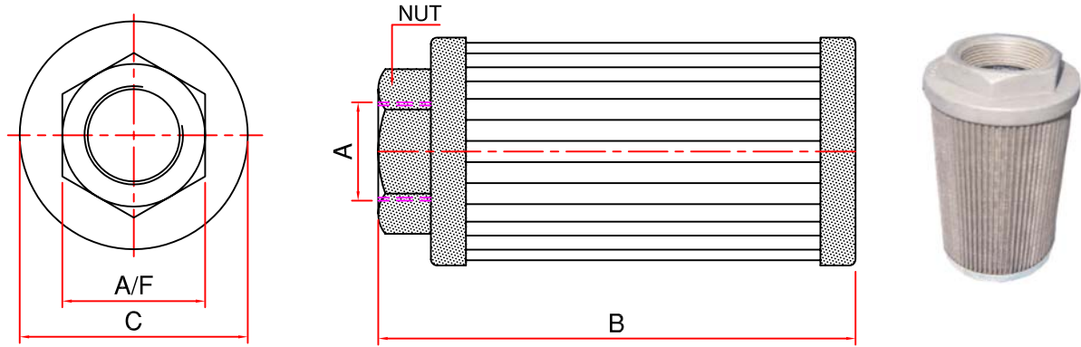
Dimensional Details
