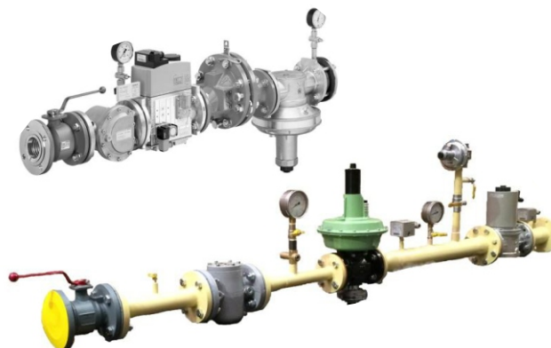
Gas Trains
