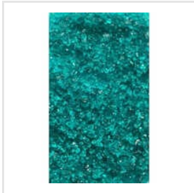
Nickel Sulfate
