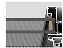
节能双层钢化中空玻璃 Energy-saving double-layer tempered insulating glass
