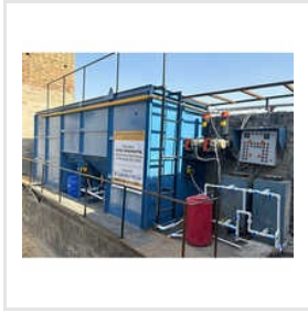
Pre Fabricated STP Plant
