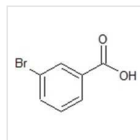
3-Bromobenzoic Acid
