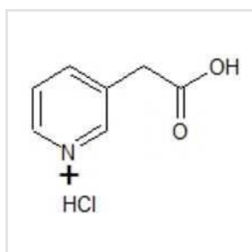
3-Pyridylacetic Acid Hydrochloride
