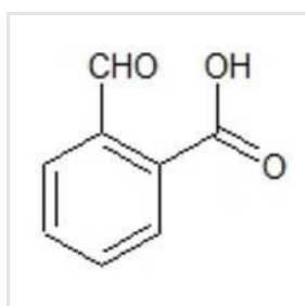
Phthalaldehyde Acid
