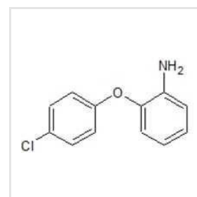
2-(4-Chlorophenoxy) Aniline
