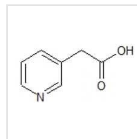
3-Pyridylacetic Acid
