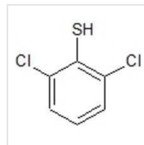
2 6-Dichloro Thiophenol
