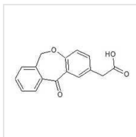
Isoxepac Acid
