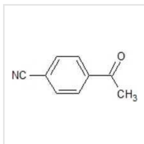
4- Acetylbenzonitrile
