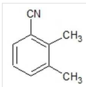
2 3- Dimethylbenzonitrile
