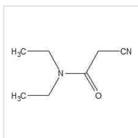
N N-Diethyl-2- Cyanoacetamide
