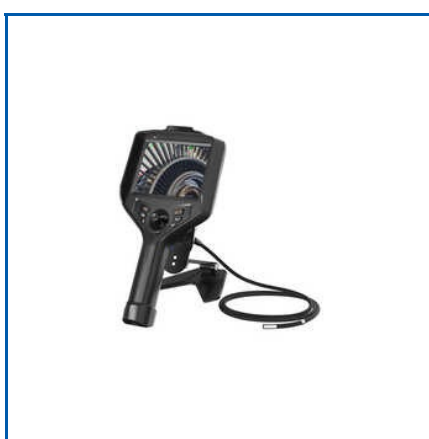
T51X SERIES 2.2MM 4-WAY ARTICULATING VIDEOSCOPE
