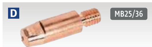
D Contact Tips MB25/36 Model No. SEE BELOW
