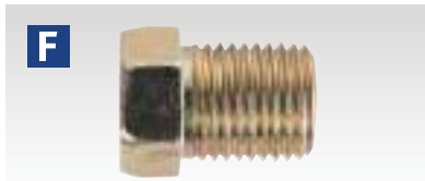
F Full Thread Male - Metric Model No. BN10100FT
