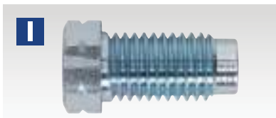
I Long Male - Imperial Model No. BN3820LM
