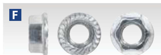
F Zinc Plated Serrated Flange Nuts DIN 6923 - M5-M12 Model No. SEE BELOW
