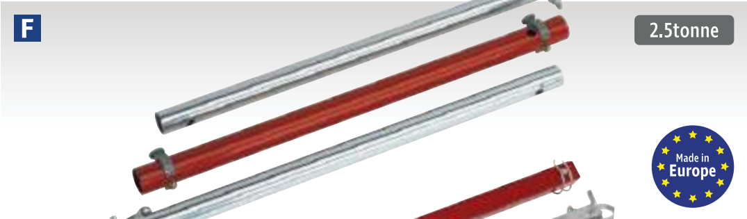
F Tow Pole 2500kg Rolling Load Capacity Model No. TPK253 2.5tonne Rolling load capacity rigid tow pole. Hook mechanism allows for mounting pole between vehicles where towing eyes may be mixed, i.e. not both horizontal or vertical. Maximum Rolling Load Capacity: 2.5tonne Length: 1.8m
