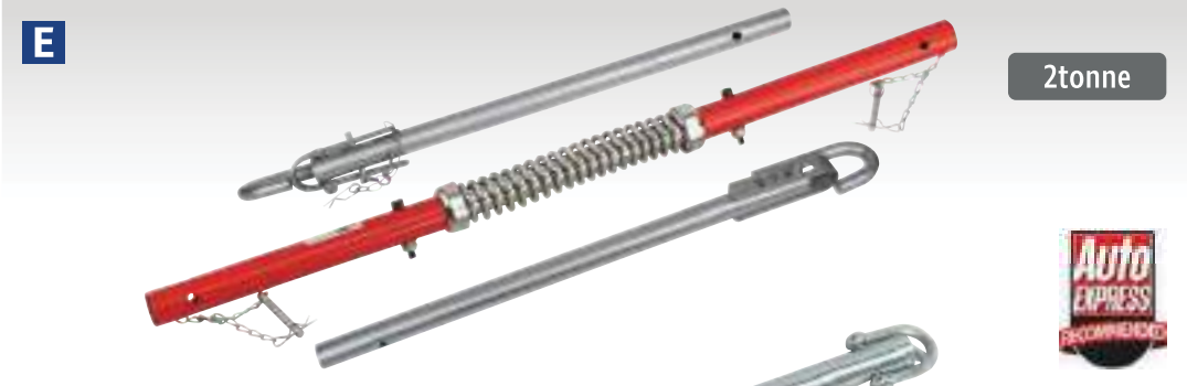
E Tow Pole with Shock Spring 2000kg Rolling Load Capacity Model No. TPK2522 2tonne Rolling load capacity tow pole with spring loaded damper unit. Locking tow hook attachment ensures secure attachment to vehicle. Suitable for mixed towing hook configurations, i.e. not both horizontal or vertical. Supplied in pouch. Maximum Rolling Load Capacity: 2tonne Length: 1.8m
