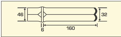
G Chisels - 1-1/4" Hex Model No. SEE BELOW
