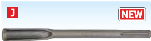
J 18 x 450mm Hollow Gouge - SDS MAX Model No. X1G
