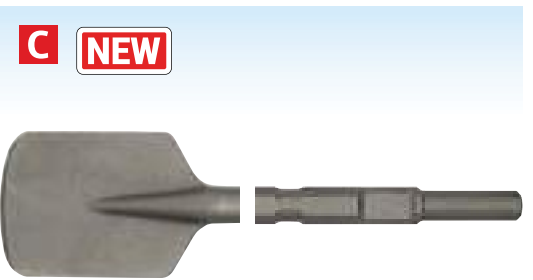
C NEW C 110 x 450mm Clay Spade - Kango 900 Model No. K1CS Length: 450mm Width: 110mm
