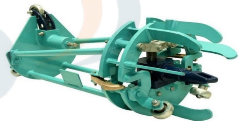
Internal Pipe Line-up Clamp
