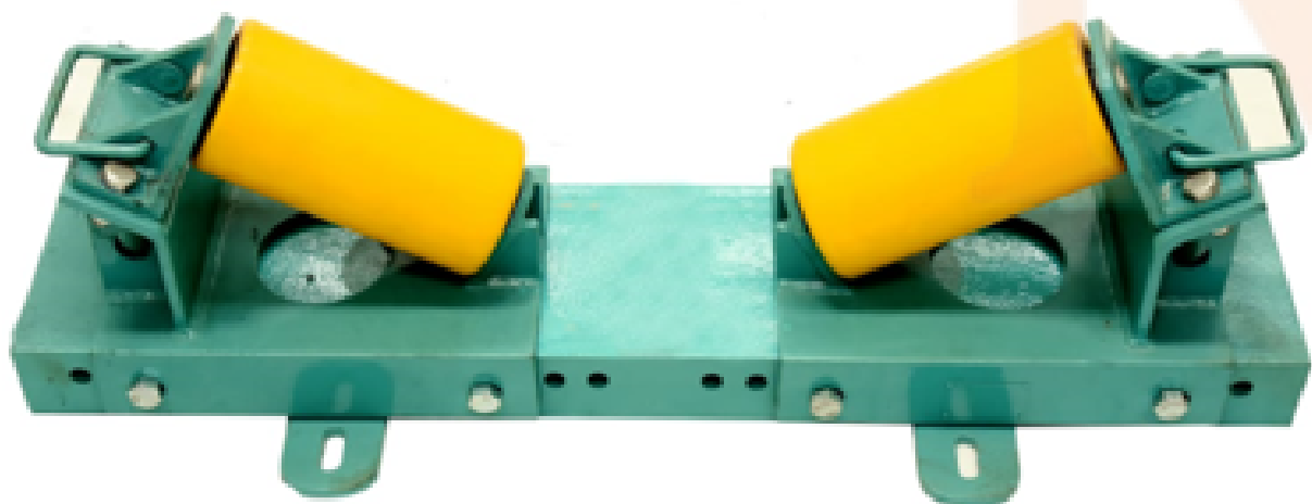
Pipe Support Rollers - Adjustable
