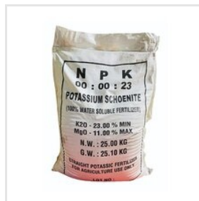
Potassium Schoenite
