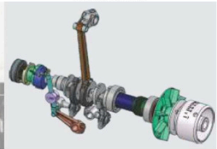
Feed Dog Angle Adjustment
