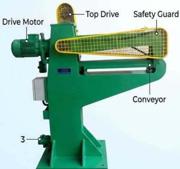
View 3: Side Profile (Conveyor End)
