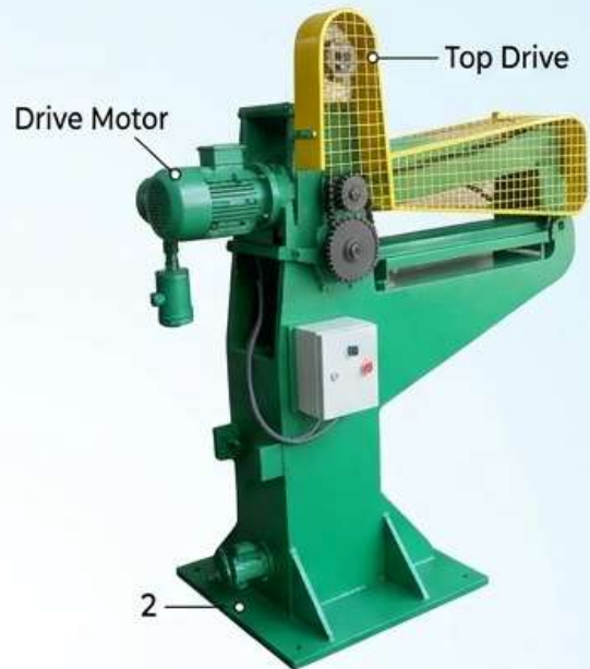
View 2: Rear View
