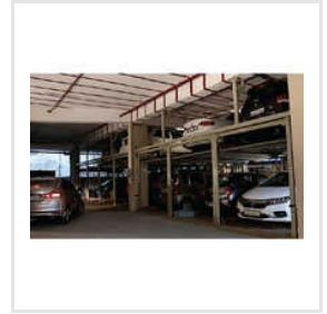
3IC-203 Puzzle Parking
