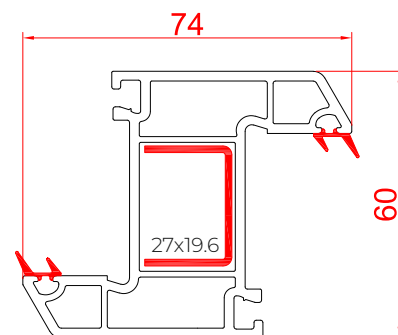
Z - Mullion - 74 RSC - 74 ZM
