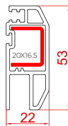
Mesh Screens Sash - 53 RSM-53M
