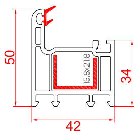
Small Casement Frame - 42 RSC-42EVF
