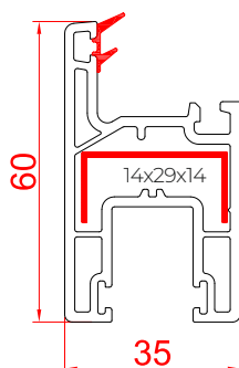
Sliding Sash - 60X35 RSS-60ES
