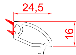
Single GLaze Bead - 24.5 RSB-24.5SB
