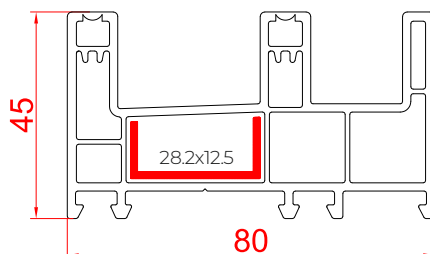
2.5 Track - 80 Series RST-80ET
