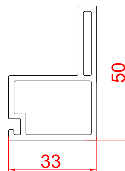
Add On Track RSA - 50 AT
