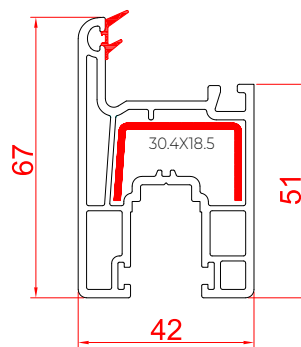
Medium Door Sash - 67 RSS-67MS
