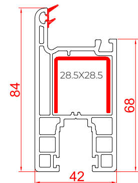
Jumbo Door Sash - 84 RSS-84BS
