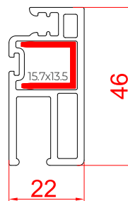
Sliding Screen Sash RSM-46EM
