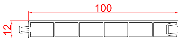
Pannel Board RSA - 12 P
