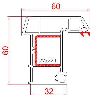
Casement Fly Mullion RSC - 60FM
