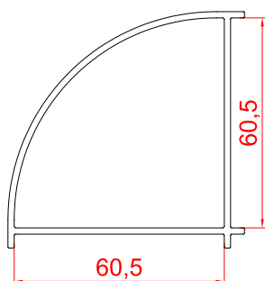
Baypole 60-60 RSA - 60B
