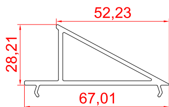
Corner Joint Copuler 60 - 112 RSA - 112 CJC
