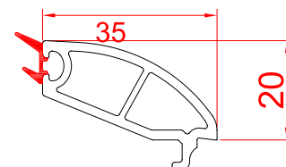
Single Glaze Casement Bead - 35 RSB - 35 CB
