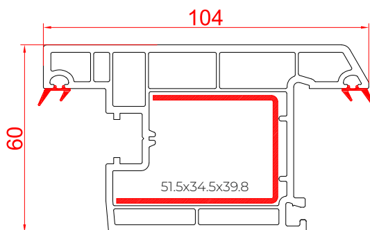
Casement Outward Door Sash RSC - 104 OD
