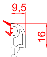
Double Glaze Bead - 9.5 RSB- 9.5 DGB
