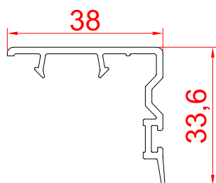
Sliding Interlock - Small RSI-38EIL
