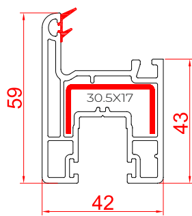
Window Sash - 59 RSS-59SS
