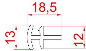
H Coupler RSA - HC
