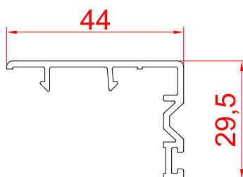
Inter Lock - 44 RSI-44IL
