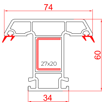
Casement T - Mullion - 74 RSC - 74 TM
