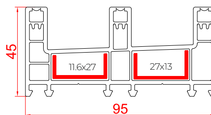
3 Track - 95 Series RST-95ET
