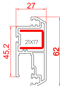
Mullion Mesh - 62 RSM-62MM
