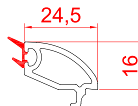
Single GLaze Bead - 24.5 RSB-24.5ESB
