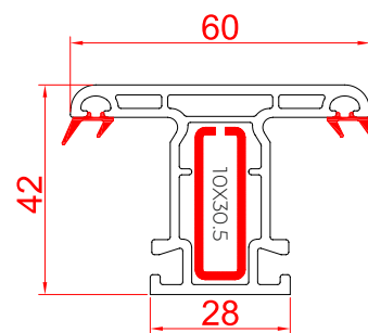
Sash Mullion - 42 RSM-42SM
