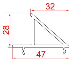
Corner Joint Copuler - 60-92 RSA - 92 CJC
