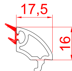
Single Glaze Bead - 17.5 RSB-17.5EB
