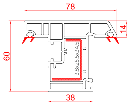
Casement Outer Sash - 78 RSC - 78 WO
