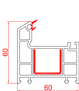
Casement Outer - 60 RSC - 60 OF
