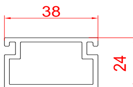
Track Connector RSA - 38 TC
