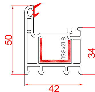
Small Casement Frame - 42 RSC - 42VF
