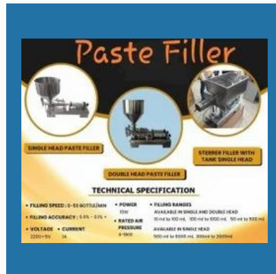
Semi Automatic Piston Filling Machine
