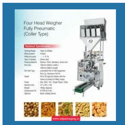
Four Head Weigher Packing Machine
