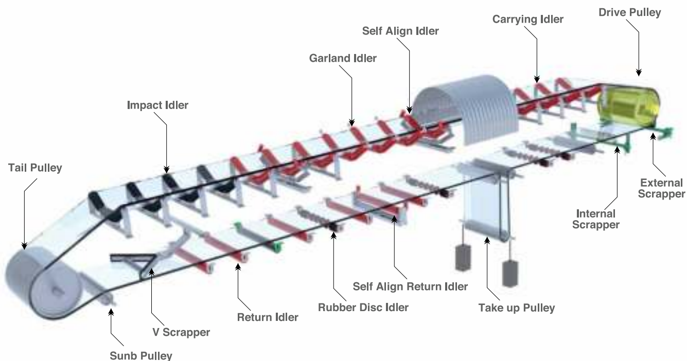
Rubber Belt
