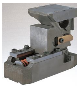
C. Cam Piercing Tools
