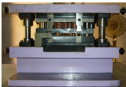
B. Radial Piercing Tools
