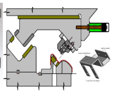
C. Cam Piercing Tools
