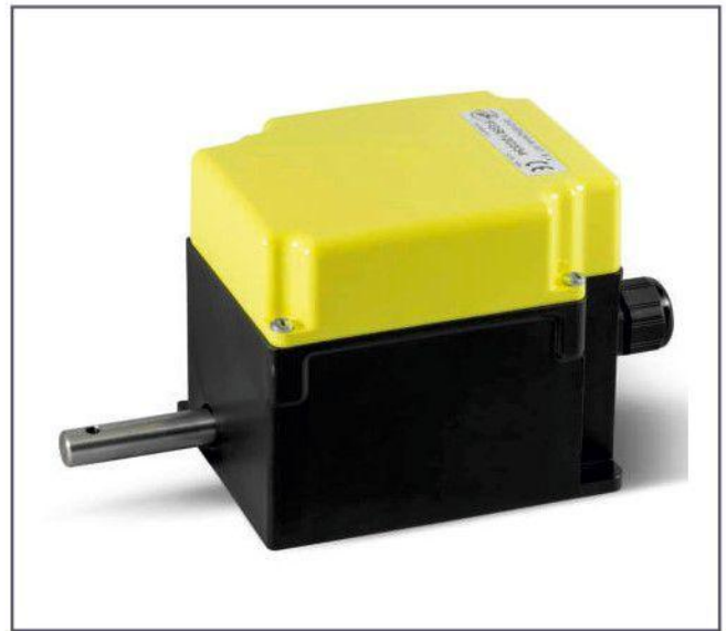
Rotary Gear Limit Switch FGR 12mm Shaft
