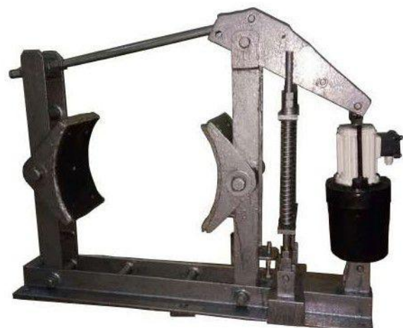
Thruster Break 500 x 46 Kg.
