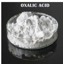
Oxalic Acid
