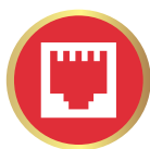
TCP/IP
