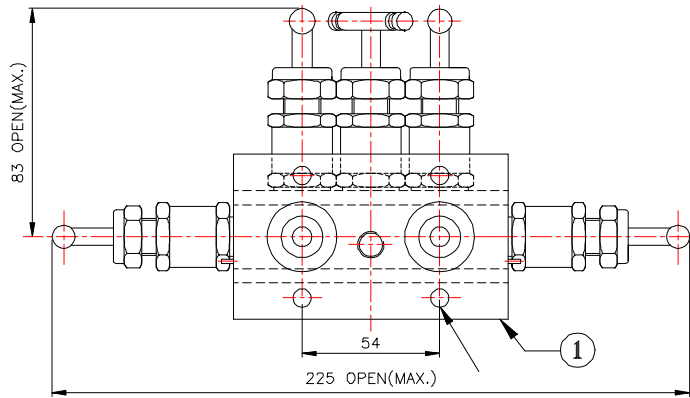
VIEW - 'BB' INSTRUMENT SIDE 4 NOS. 12.5mm. DIA MOUNTING HOLE.
