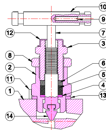
BONNET ASSEMBLY
