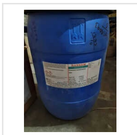
Potassium Metabisulfite
