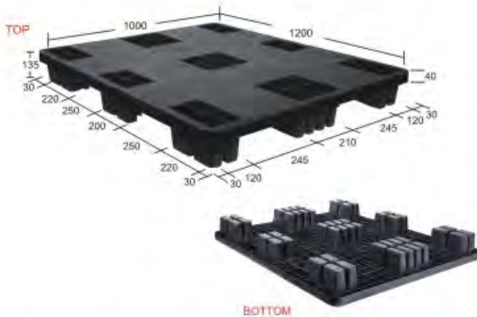
Model: SIM1210135 PPDN 9L (Supreme Injection Moulded Partially Perforated Deck Nestable 9 Legs)
