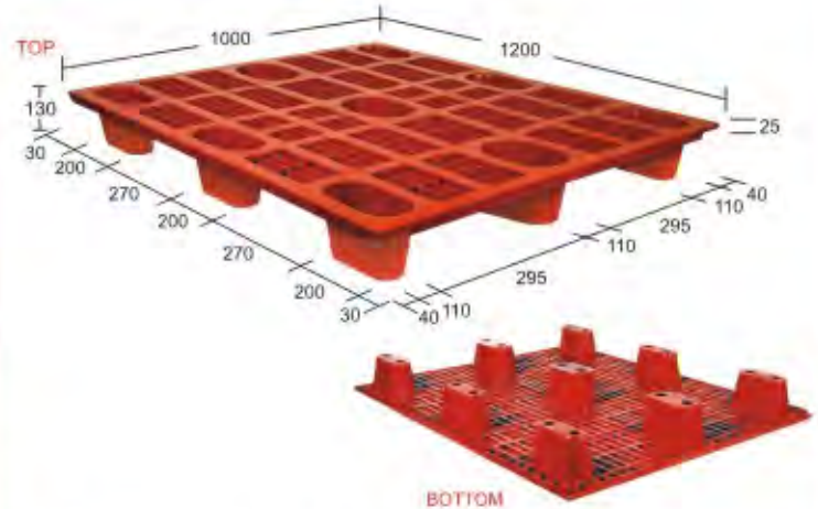
Model: SIMEXP121013 PDN 9L (Supreme Injection Moulded Export Purpose Perforated Deck Nestable 9 Legs)
