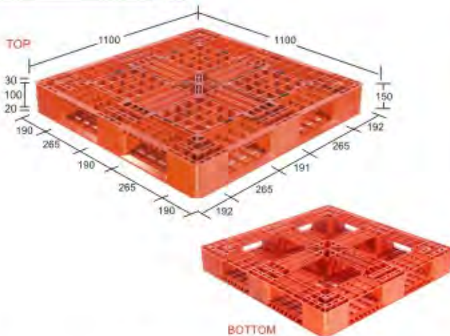
Model: SIMEXP111115 PDD (Supreme Injection Moulded Export Purpose Perforated Double Deck)
