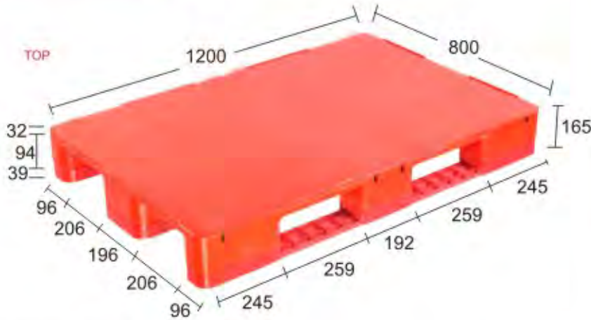
Model: SIM1280165 CDSS 3S (Supreme Injection Moulded Three Runner Close Deck Single Side with 3 Detachable Skids)
