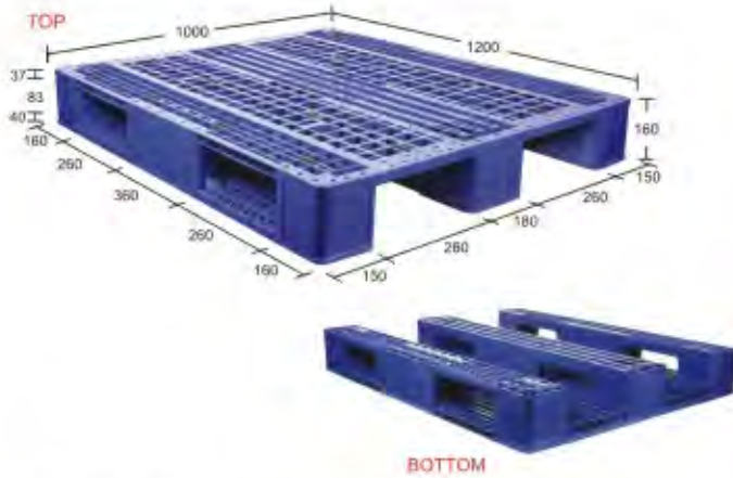
Model: SIM121016 PDSS (Supreme Injection Moulded Three Runner Perforated Deck Single Side)
