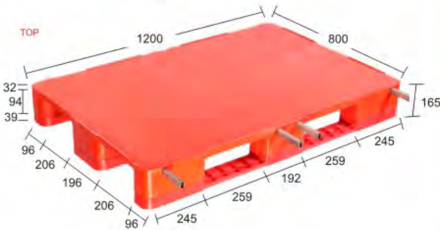
Model: SIM1280165 CDSS SR 3S (Supreme Injection Moulded Three Runner Steel Reinforced Close Deck Single Side with 3 Detachable Skids)
