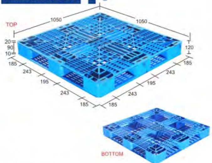
Model: SIMEXP105105 PDD (Supreme Injection Moulded Export Purpose Perforated Double Deck)
