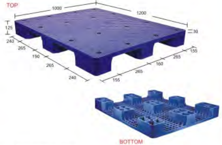
Model: SIM1210125 CDSS 9L (Supreme Injection Moulded Close Deck Single Side 9 Legs)
