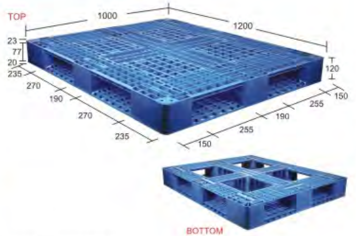
Model: SIM121012 PDD LW (Supreme Injection Moulded Perforated Double Deck Light Weight)
