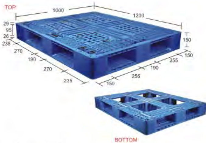
Model: SIM121015 PDD MW (Supreme Injection Moulded Perforated Double Deck Medium Weight)
