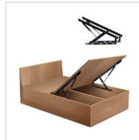
Heavy Duty Bed Non-Lockable Gas Spring
