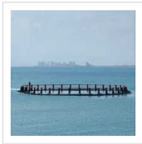
16 Diameter HDPE Circular Cage
