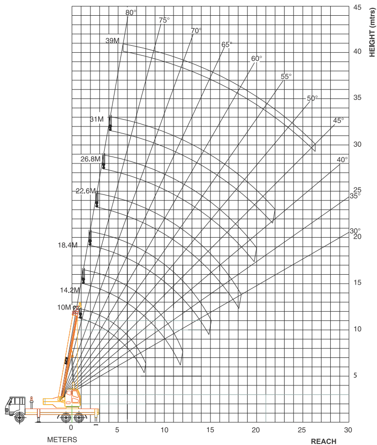
Lifting dimensions
