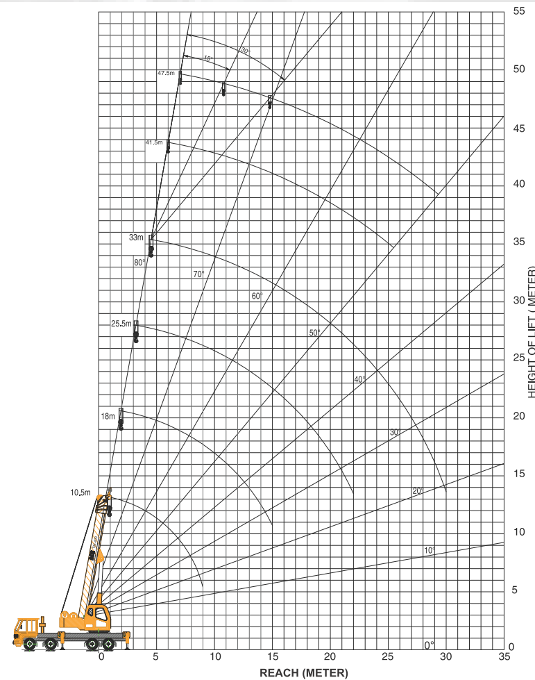
Working Range
