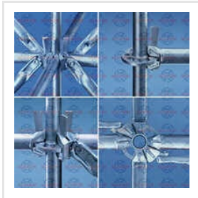
Ring Lock
