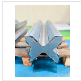
Bending Dies
