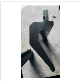
Gooseneck Punch For Press Brake
