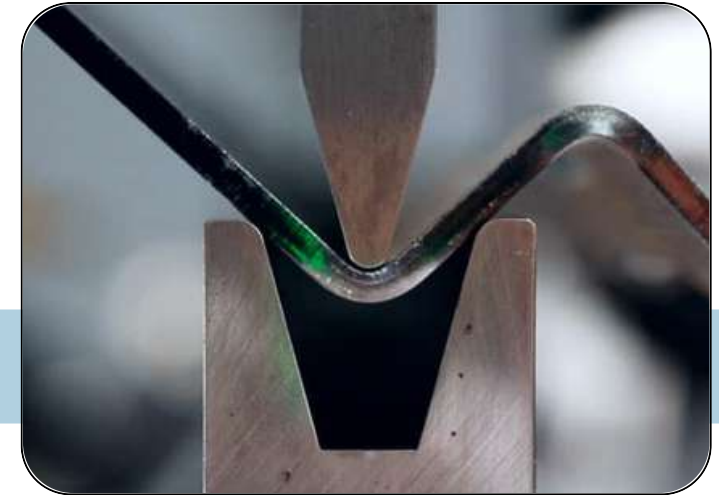
CNC BENDING SERVICES
