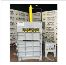
Industrial Cardboard Baler Machine
