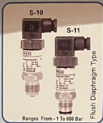
Pressure Transmitter
