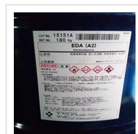
ETHYLENEDIAMINE (EDA)
