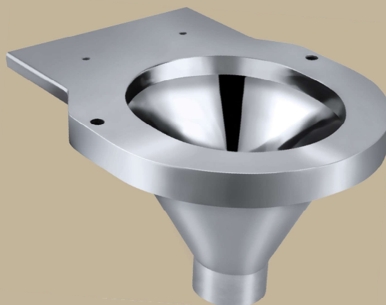
STAINLESS STEEL EURO BOWL ASSEMBLY FOR RAILWAY (DRG No.: LS63117)
