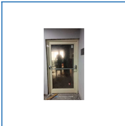
84 INCH GLAZED FIRE RATED STEEL DOOR
