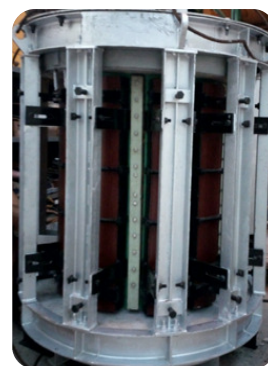
Coil Cradle Assembly
