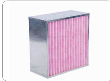
Panel Type Air Filter
