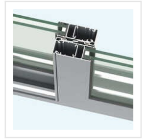
29mm Ventana Series Aluminium Profile
