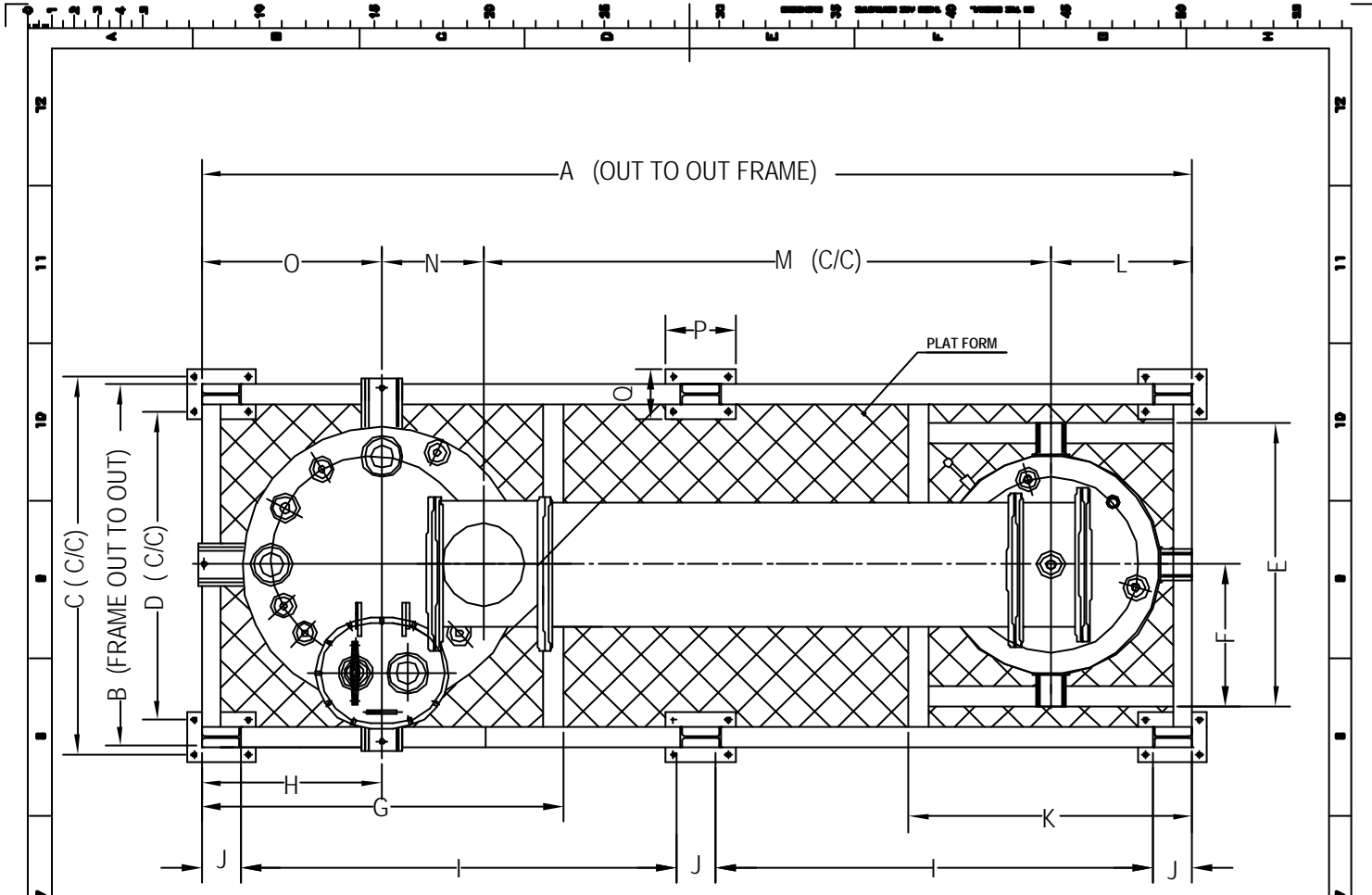
STRUCTURE LAY OUT (TOP - VIEW) VIEW OF DISTILLATION PLANT
