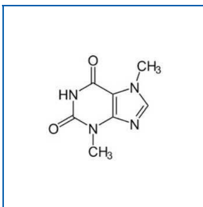
THEOBROMINE
