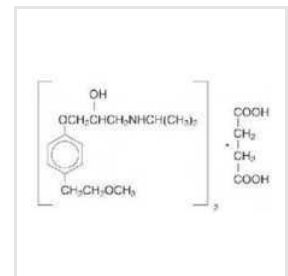
METOPROLOL SUCCINATE
