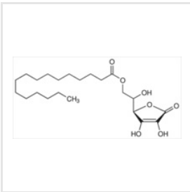
Ascorbyl Palmitate
