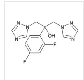
Fluconazole
