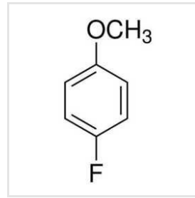
4-Fluoroanisole
