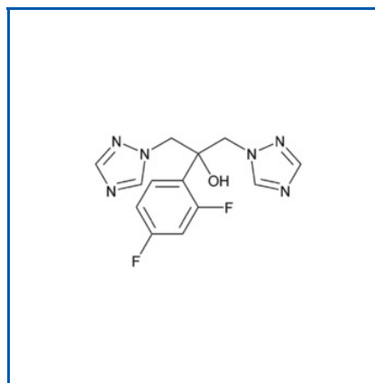
FLUCONAZOLE
