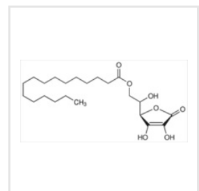
Ascorbyl Palmitate
