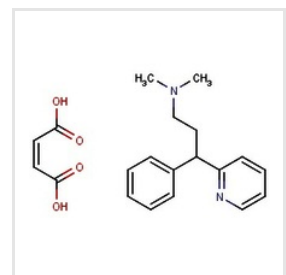
Pheniramine Maleate
