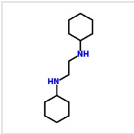
N,N'-Dicyclohexyl-1,2-Ethanediamine
