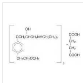
METOPROLOL SUCCINATE
